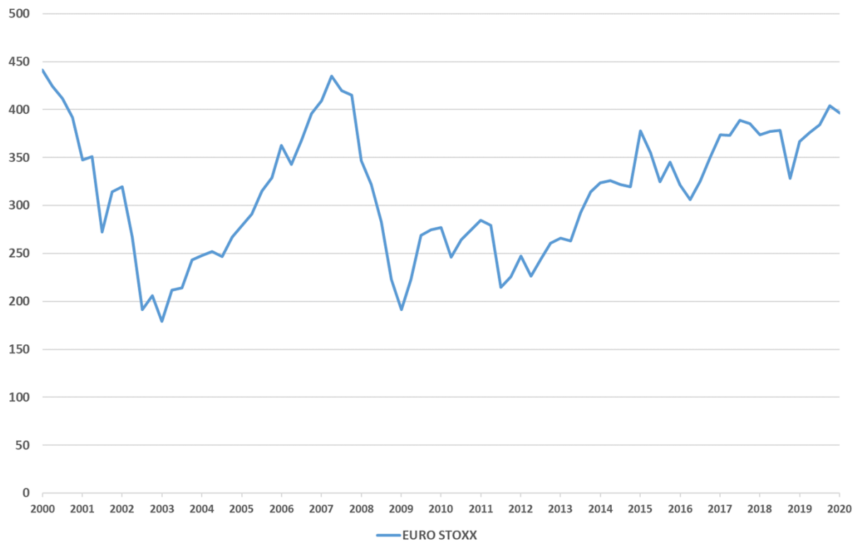
Figure 28: EuroStoxx index 2000-2020
